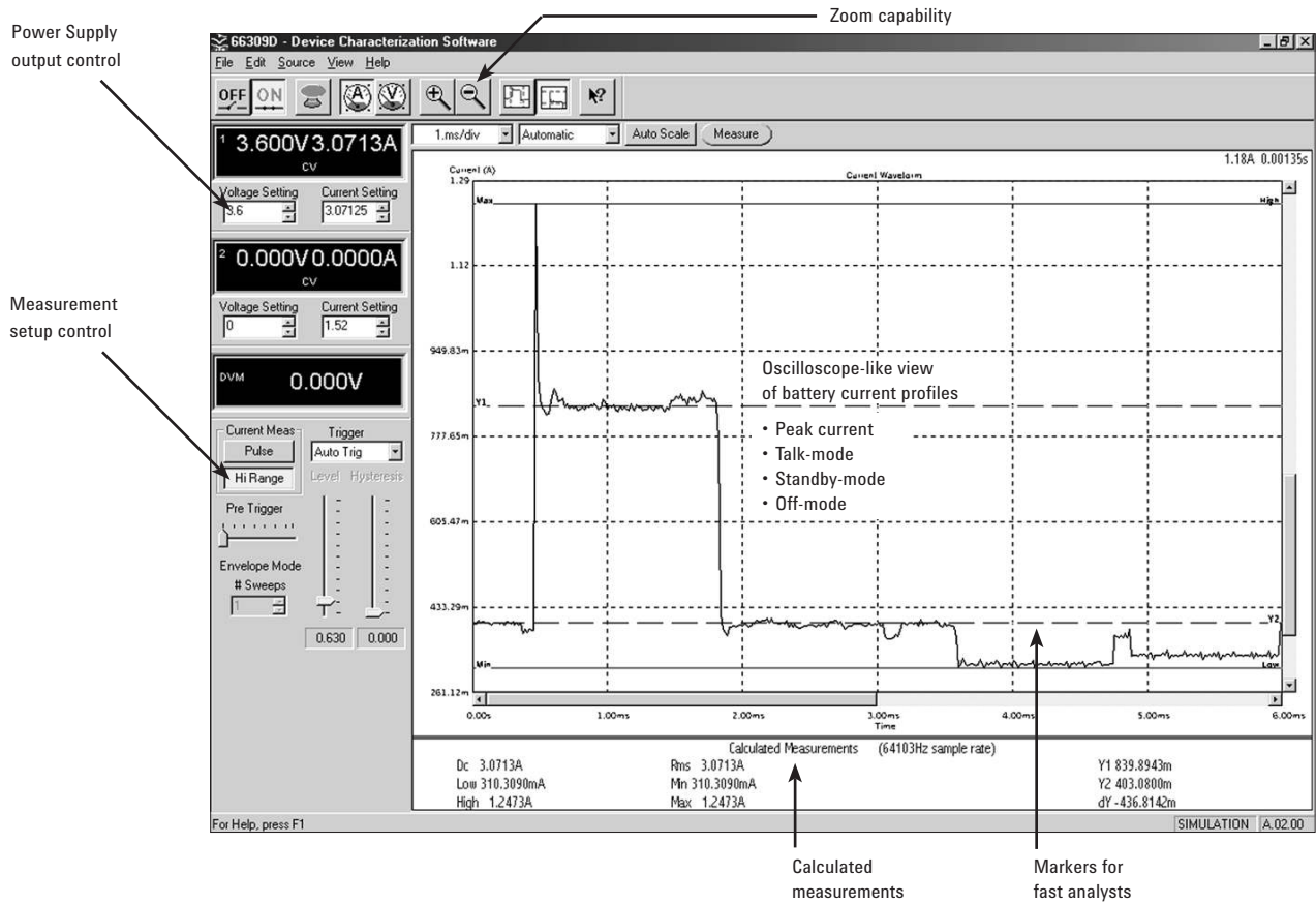
Figure 9. 14565B Device Characterization Software displaying GSM pulse current waveform
